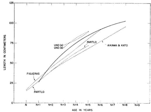
FIG. 8. A comparison of the growth curves obtained by the vertebral method with the Walford curve obtained in this study. Specific ages are disregarded in the plotting of these curves.
