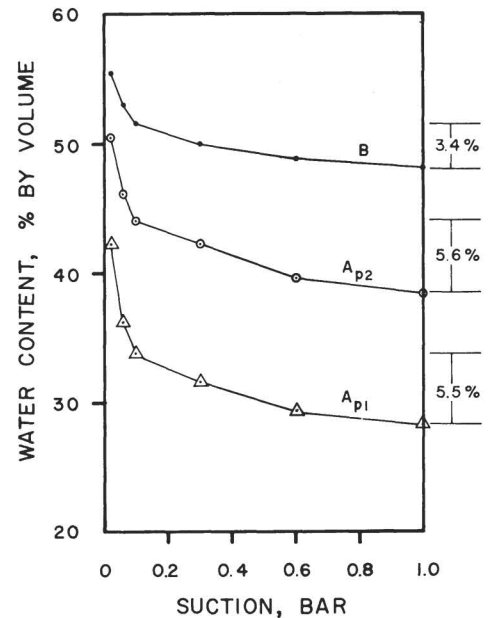
Fig. 2. Water-retention curves for a Haiku clay.
