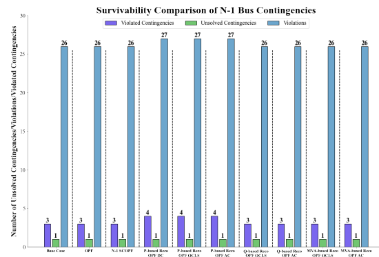
(b) N-1 Bus Contingencies
