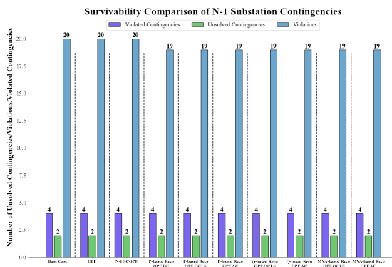
(c) N-1 Substation Contingencies
