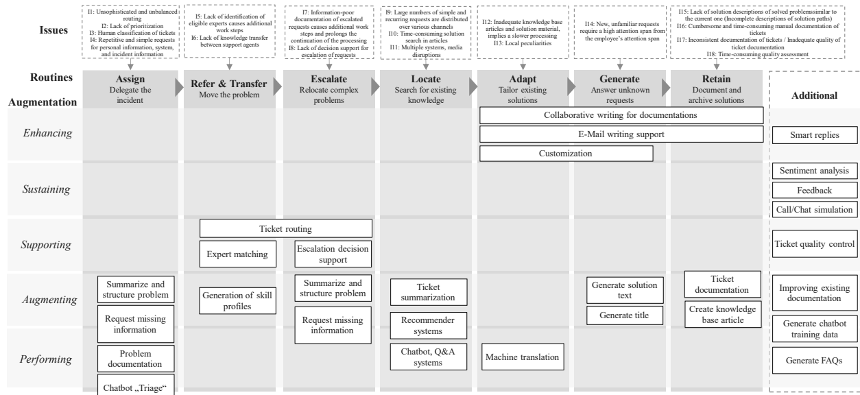
Figure 3: Routine-based AI augmentation framework for customer support services.
