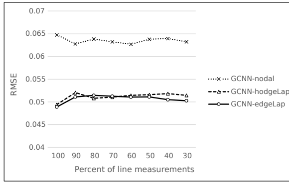
Figure 5: This figure compares the performance of state estimation for the IEEE 57 bus system between three methods: GCNN-nodal, GCNN-hodgeLap and GCNN-edgeLap.
