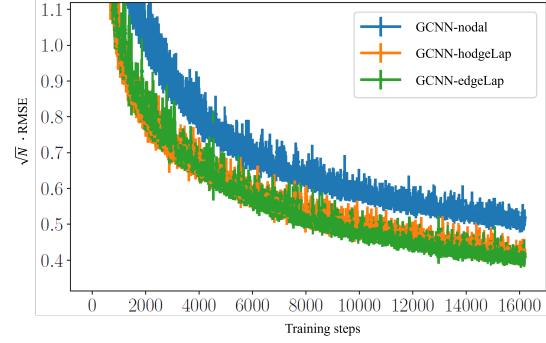
Figure 1: RMSE values in the validation stage for the IEEE 57-bus test case. It is observed that with the progression of training steps (parameter updates through ADAM), the RMSE lowers, showing that the GCNNs are indeed learning.
