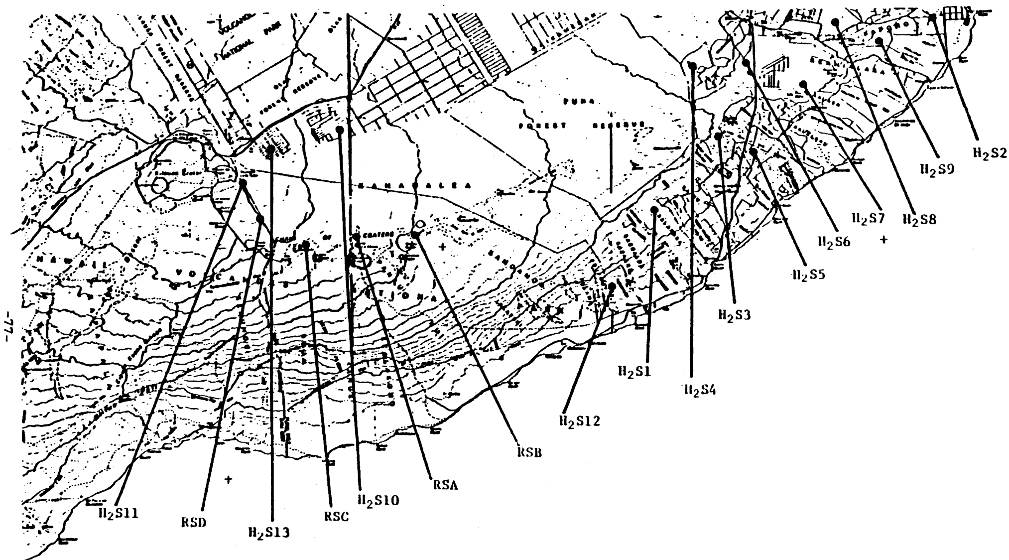
Figure 8. Approximate Location of Passive H_2S , Radon, and SFU Monitoring Stations ( H_2S1 - H_2S13 and RSA-RSD). (SFU-stacked filter unit) Source: Houck, 1984
