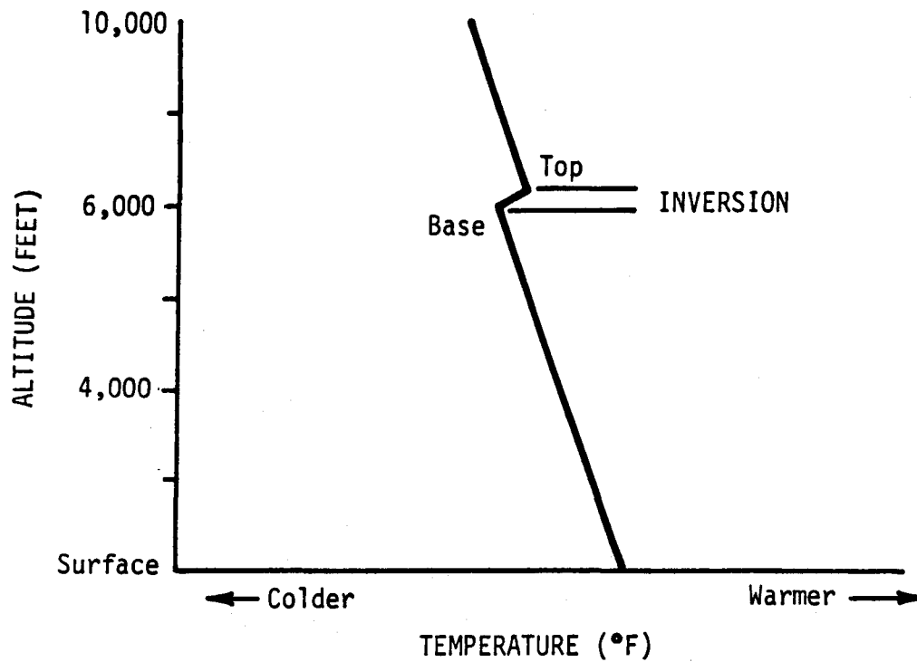
Figure 3a. Trade wind Temperature Inversion
