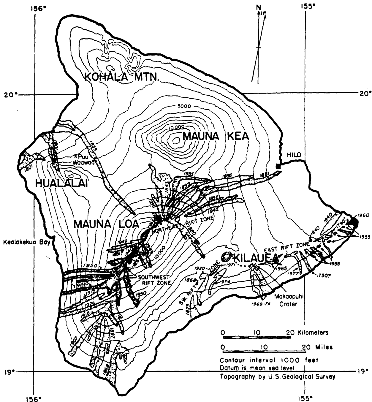
Figure 8. Map of the island of Hawaii, showing the five major volcanoes that make up the island, and the historic lava flows. (Macdonald et al., 1983)
