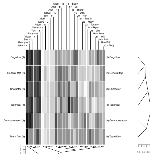
Figure 2 Aggregate RepGrid
