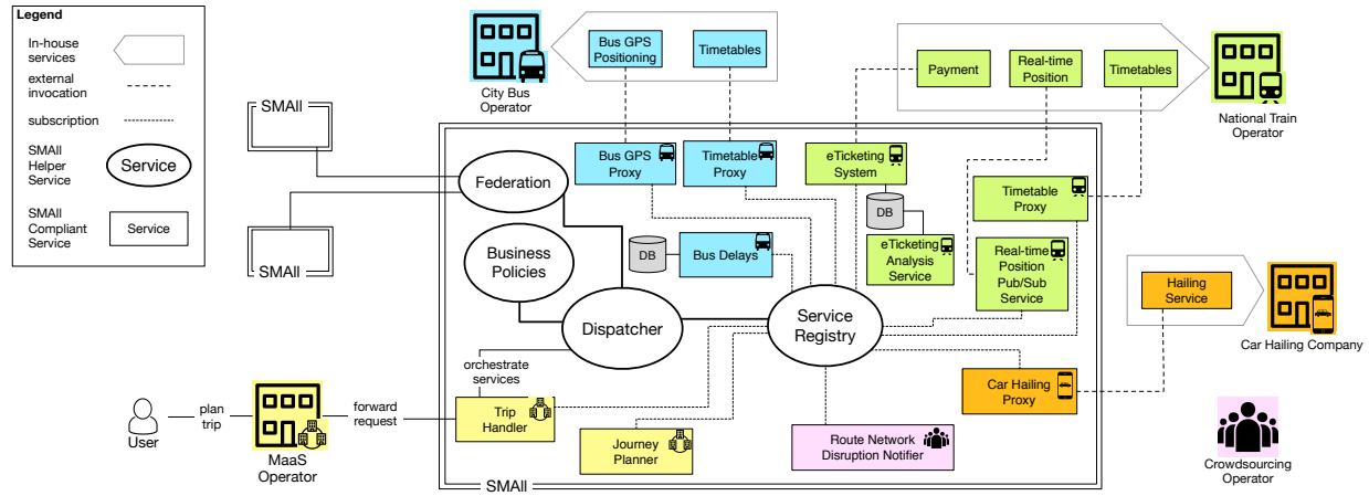
Figure 1. Example of the SMAII architecture.
