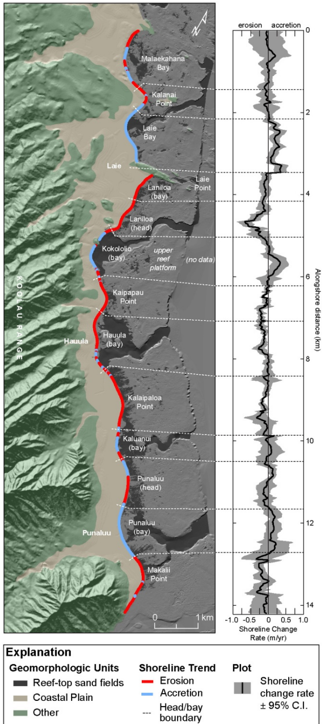
Figure 4.5. Shoreline change trends for the beaches of Malaekahana through Makalii Point, northeast Oahu, Hawaii (see Figure 4.1 for location). Historical shoreline trends (plot, color-coded alongshore bars) indicate greater erosion along headland beaches than along beaches within embayments. The surficial geology of the low-lying coastal plain (tan) is primarily Holocene carbonate beach deposits and alluvium (Sherrod et al. , 2007). Locations of reef-top sand deposits are adapted from Conger (2009) and visual interpretation of aerial photographs and bathymetric models.
