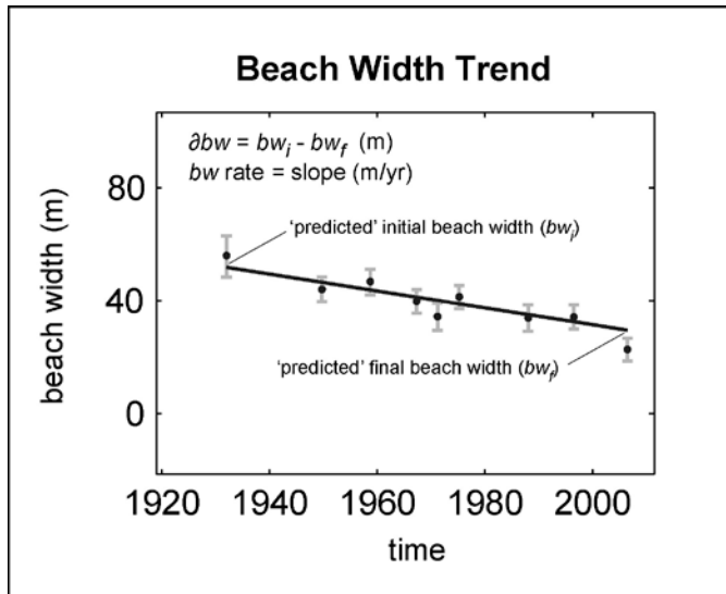
Figure 2.3. Calculating beach width change with weighted least squares (WLS). Regional average beach widths, average beach width changes, and average beach width rates are the average of values from all transects in a beach section. Following Equation 9 of Hapke et al. (2010), the uncertainty of regional averages are estimated using an effective number of independent uncertainty observations ( n^* ), calculated using a spatially-lagged (along-shore) autocorrelation of the uncertainty values.
