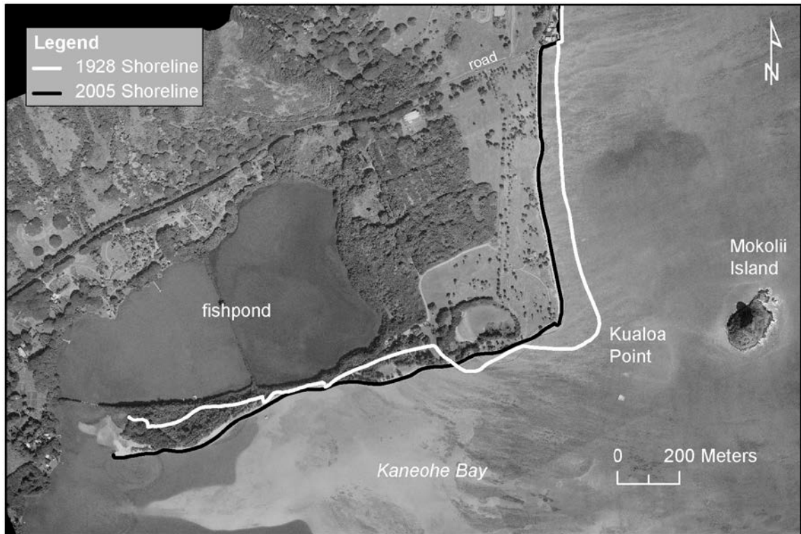
Figure 4.8. Aerial photograph (2005) and historical shoreline positions (1928 and 2005) documenting erosion along the headland beach at Kualoa Point, east Oahu, Hawaii (see Figure 4.1 for location). Note the accretion cusp within Kaneohe Bay formed by eroded sand transported into Kaneohe Bay from Kualoa Point.
