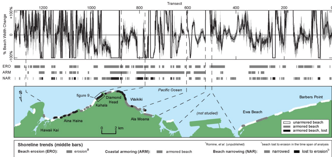
Figure 2.8. South Oahu beach width percent changes (plot, 1928 or 1949 to near present), shoreline trends (middle bars), and coastal armoring (map).
