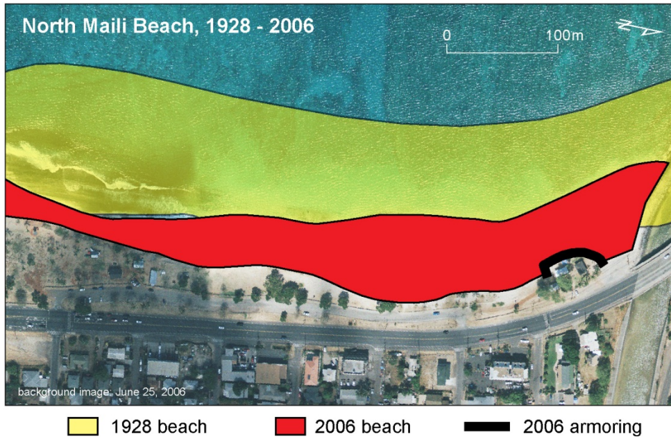
Figure 2.12. In spite of shoreline recession of over 100 m, substantial beach remains along the (mostly) unarmored northern end of Maili Beach (1928-2006, location shown in Figure 2.11).
