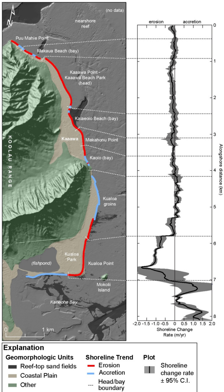
Figure 4.6. Shoreline change trends for the beaches of Kaaawa through Kualoa Point, northeast Oahu, Hawaii (see Figure 4.1 for location). Historical shoreline trends (plot, color-coded alongshore bars) indicate greater erosion along headland beaches than along beaches within embayments. Note: shoreline trends for Kualoa ('Kualoa groins' through Kualoa Point) are not included in overall shoreline change analysis for northeast Oahu (Table 4.1). Accretion within the Kualoa groins is due largely to efforts to stabilize the shoreline with engineered structures. The surficial geology of the low-lying coastal plain (tan) is primarily Holocene carbonate beach deposits and alluvium (Sherrod et al. , 2007). Locations of reef-top sand deposits are adapted from Conger (2009) and visual interpretation of aerial photographs and bathymetric models.
