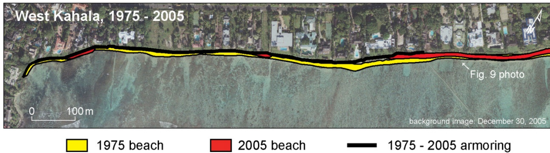
Figure 2.9. Beach loss at Kahala, south Oahu (1975-2005, location shown in Figure 2.8).
