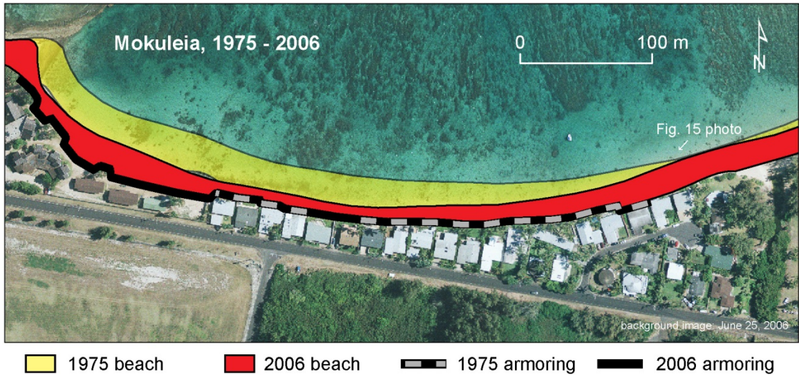
Figure 2.14. Beach narrowing and flanking erosion at Mokuleia, north Oahu, as of June, 2006 (1975-2006, location shown in Figure 2.13).
