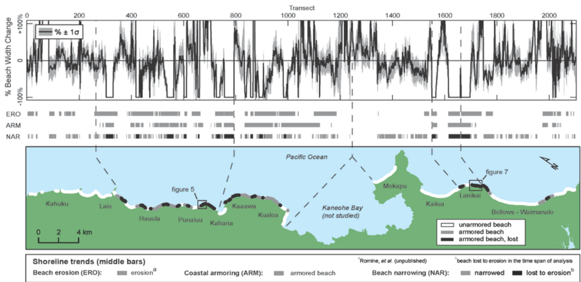
Figure 2.4. East Oahu beach width percent changes (plot, 1928 or 1949 to near present), shoreline trends (middle bars), and coastal armoring (map).
