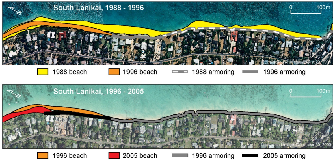
Figure 2.7. Beach loss and flanking erosion at south Lanikai (1988-2005, location shown in Figure 2.4).
