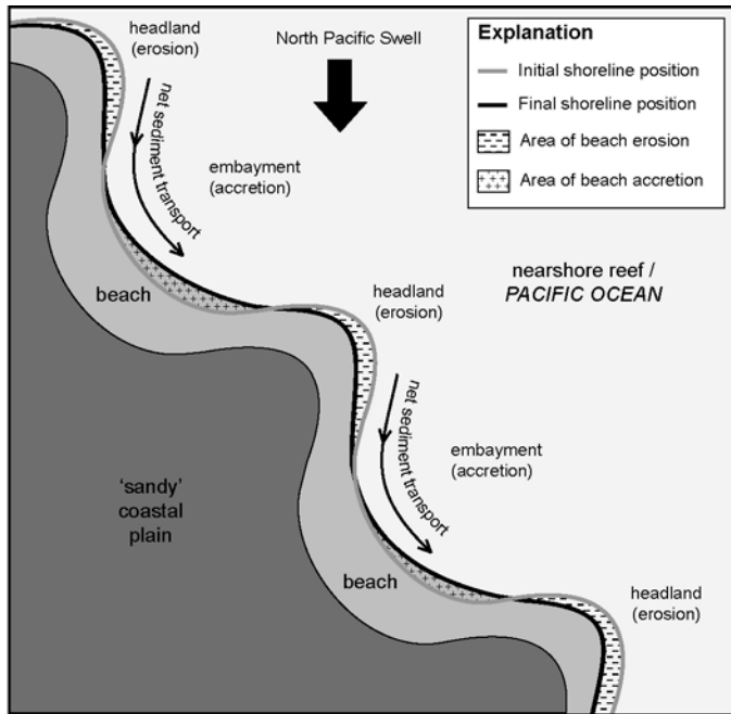
Figure 4.10. Conceptual diagram of erosion and accretion trends and inferred net sediment transport between Laniloa Beach and Makalii Point (see Figure 4.5 for location).
