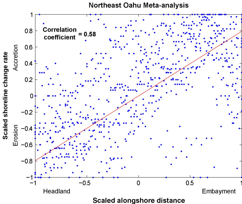
Figure 4.7. Meta-analysis of scaled shoreline change rates and alongshore distance for embayed and headland beach segments of northeast Oahu indicates a correlation between headland erosion and embayment accretion (correlation coefficient = 0.58, regression line shown in red).
