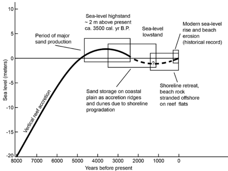
Figure 4.3. Conceptual Holocene sea-level curve for Oahu (adapted from Fletcher et al. (2008)) indicating sea level ~2 m higher than present ca. 3500 years BP, followed by a period of falling sea level prior to the initiation of modern sea-level rise observed in tide gauge records.
