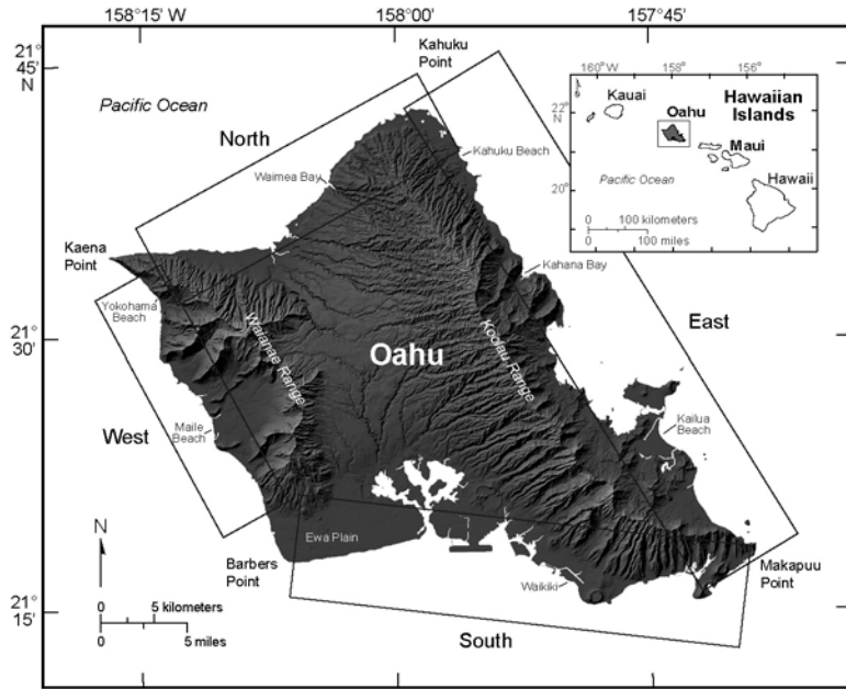
Figure 3.1. Oahu island, Hawaii, showing four beach study regions: north, east, south, and west.
