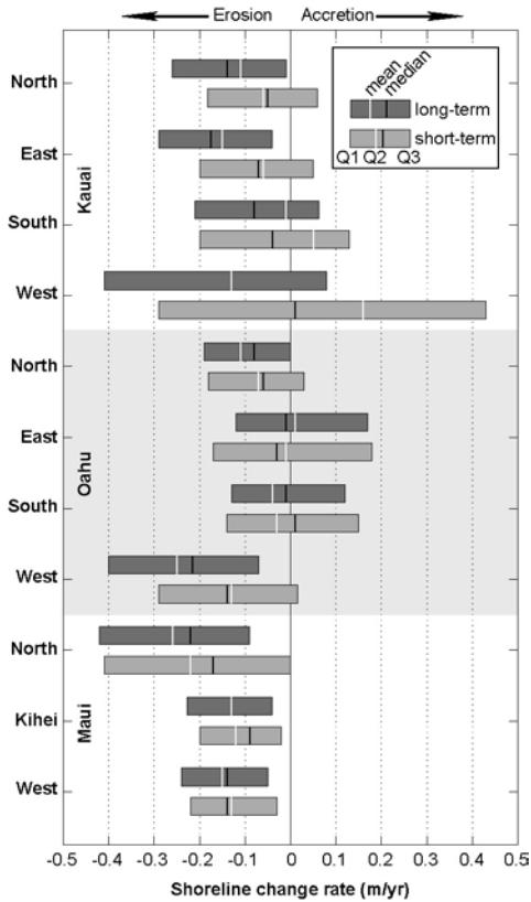
Figure 1.4. Box plot of long- and short-term shoreline change rates for coastal regions of Kauai, Oahu, and Maui. The width of a box depicts the upper and lower quartiles (Q1 and Q3) of the distribution of shoreline change rates for a region (i.e., the middle 50% of the data). Results outside Q1 and Q3 are not shown.
