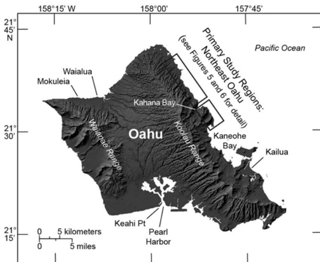
Figure 4.1. Map of study locations on the island of Oahu, Hawaii. The black boxes outline the primary study regions along the northeast Oahu coast.
