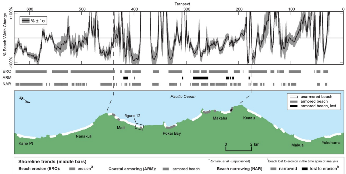
Figure 2.11. West Oahu beach width percent changes (plot, 1928 or 1949 to near present), shoreline trends (middle bars), and coastal armoring (map).
