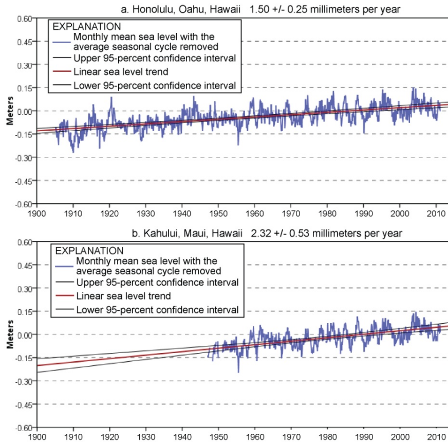
Figure 3.3. Mean sea-level trends at a. Honolulu, Oahu 1905-2011; and b. Kahului, Maui 1947-2011 ( http://tidesandcurrents.noaa.gov ).
