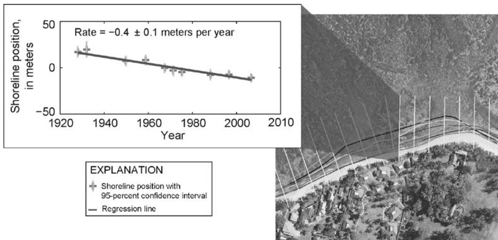
Figure 1.3. Historical shorelines (shore-parallel lines) are measured at regularly-spaced transects (roughly shore-perpendicular lines, ~20 m spacing). Shoreline change rates are calculated using weighted least squares (WLS) linear regression.
