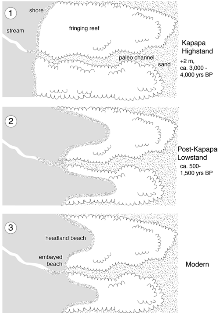
Figure 4.11. Conceptual illustration of inferred late-Holocene shoreline change regimes along the northeast coast and elsewhere on Oahu. The Kapapa sea-level high stand (ca. 3,500 yr BP, approx. +2 m) resulted in an overall trend of shoreline recession. A post-Kapapa sea-level low stand (ca. 500 – 1,500 yr BP) resulted in increased progradation (accretion) of headland beaches fronting shallow reef, relative to embayed beaches fronting channels, creating a sinuous beach morphology. Modern sea-level rise has resulted in a change in shoreline regimes to “preferential” erosion along headland beaches and in-filling (accretion) at embayed beaches.
