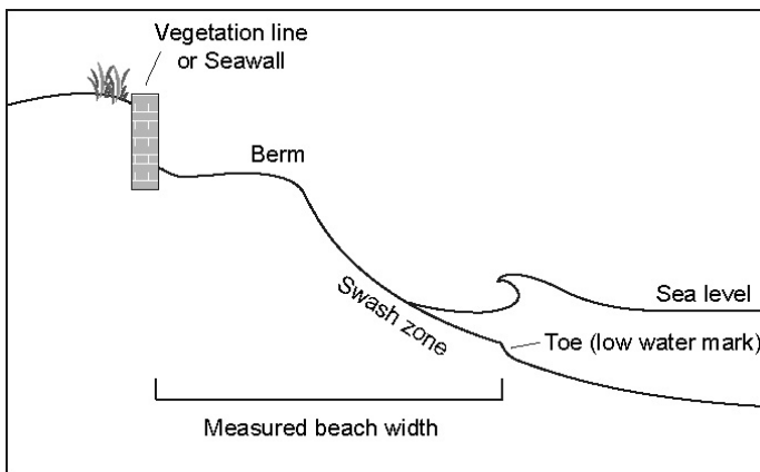
Figure 2.2. Beach width is the distance between the beach toe (low water mark) and vegetation line (or armoring) (modified from Fletcher, et al. (1997)).
