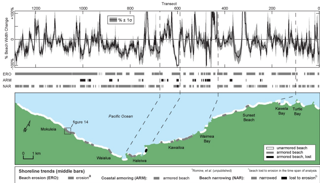
Figure 2.13. North Oahu beach width percent changes (plot, 1928 or 1949 to near present), shoreline trends (middle bars), and coastal armoring (map).
