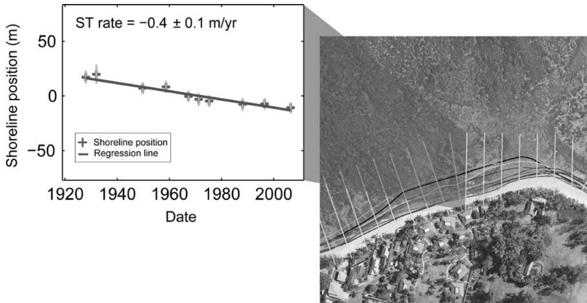
Figure 3.4. Calculating shoreline change rate from historical shoreline positions with the single-transect (ST) method (using weighted least squares, WLS). Historical shoreline positions and transect locations are shown on a portion of a recent aerial photograph.
