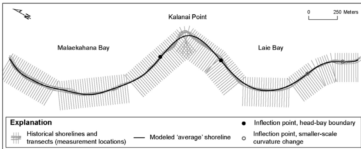
Figure 4.4. To delineate headland beaches and embayed beaches, a polynomial shoreline model (Legendre Polynomial) is fit to historical shoreline positions with least squares regression. Boundaries between headlands and bays are located by differentiation of the shoreline model to identify inflection points (changes in curvature) between headland (convex seaward) beach sections and embayed (concave seaward) beach sections (example shown from Malaekahana and Laie Bays, northeast Oahu).
