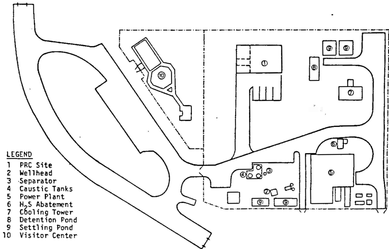
Figure 4. Schematic of HGP-A Site
