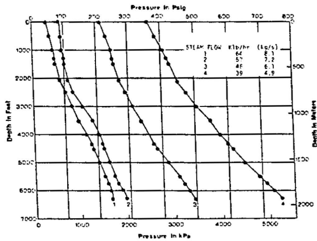
Figure 6. Pressure Profiles in HGP-A [1,2]
