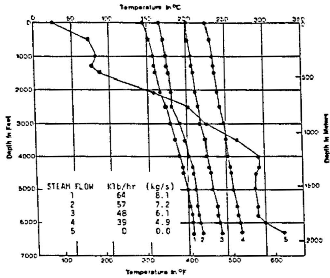
Figure 5. Temperature Profiles in HGP-A [1,2]
